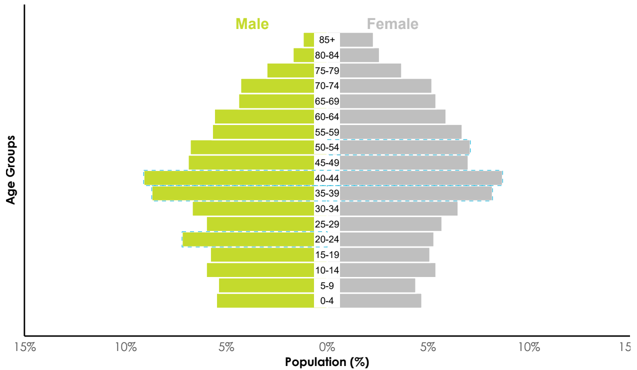
Figure 3: Population pyramid (%)
